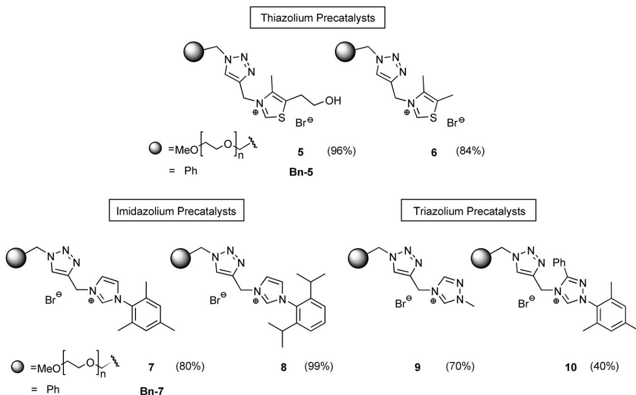
Figure 1. 1,2,3-Triazolo-linked heterazolium precatalysts (loading in %).
