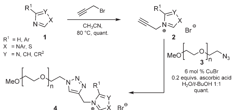
Scheme 1. Synthesis of supported heterazolium precatalysts via “CuAAC”.
